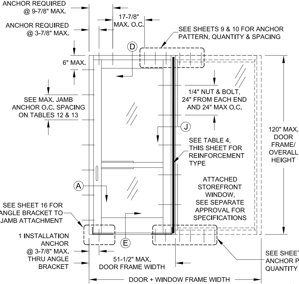
TYP. ELEVATION OF SINGLE DOOR WITHOUT TRANSOM
