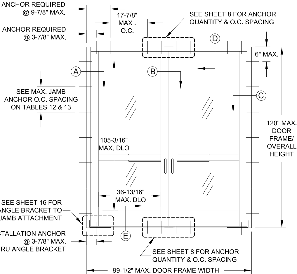
TYP. ELEVATION OF DOUBLE DOOR WITHOUT TRANSOM
