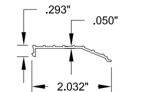
16 ADA THRESHOLD COVER (1/2" TOTAL SILL HEIGHT)
