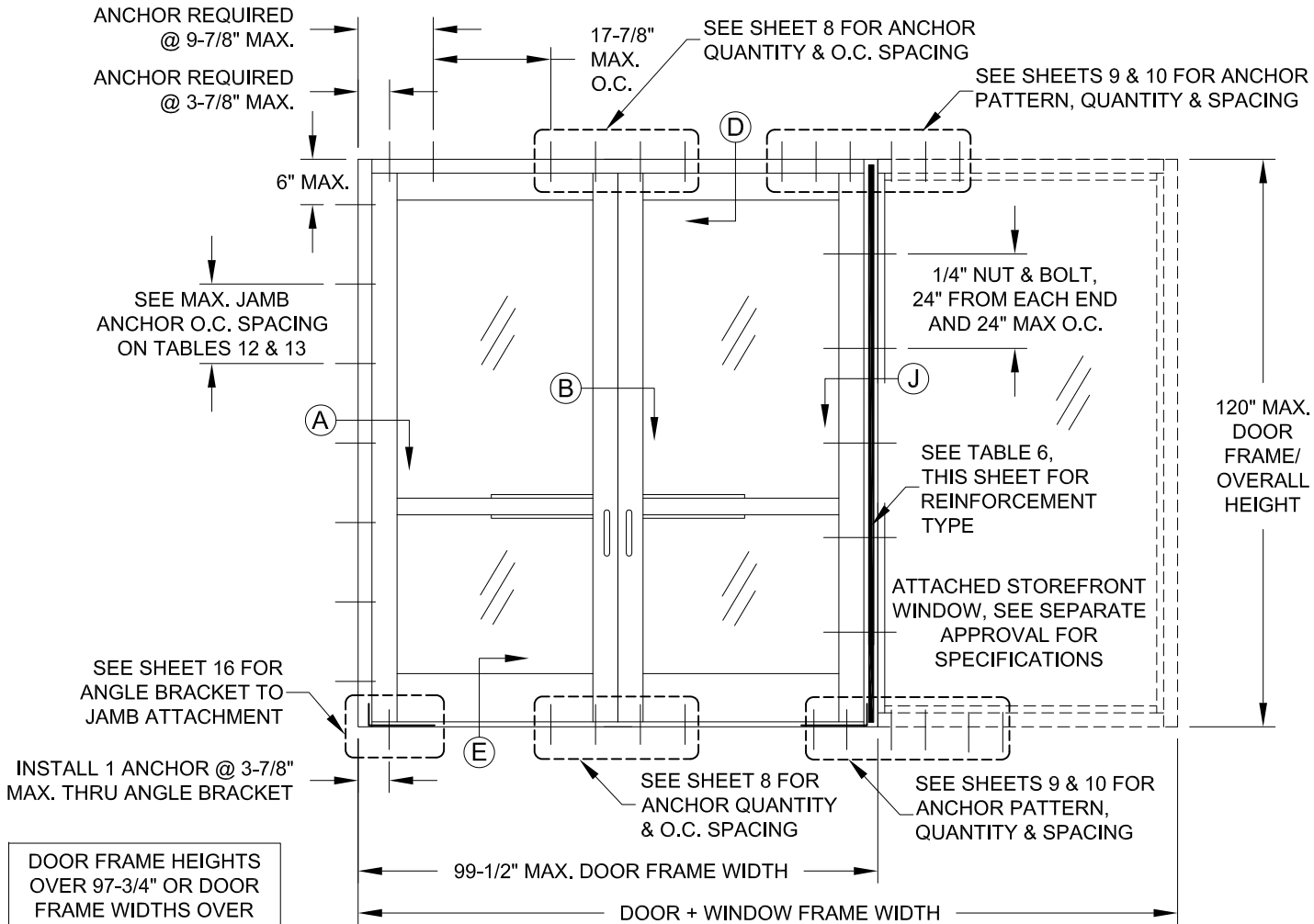
TYP. ELEVATION OF DOUBLE DOOR WITHOUT TRANSOM, ATTACHED TO STOREFRONT WINDOW
