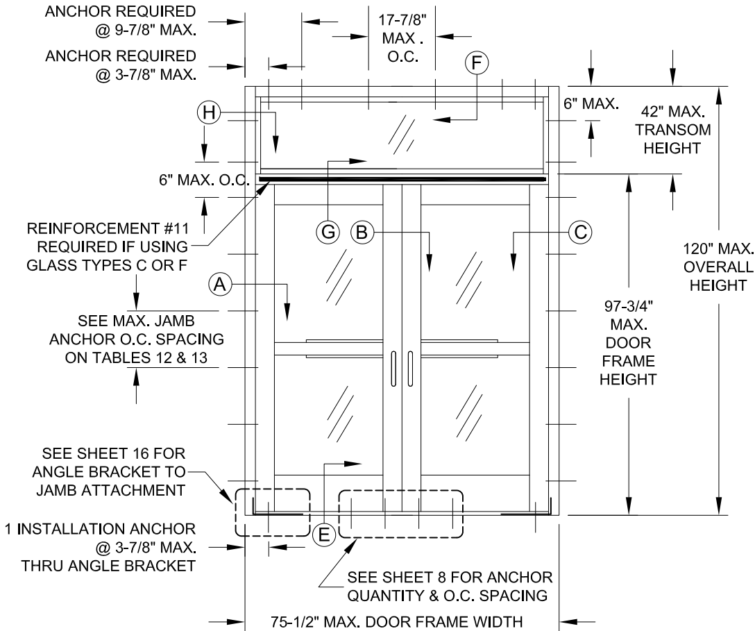
TYP. ELEVATION OF DOUBLE DOOR WITH TRANSOM
