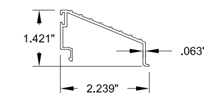
17 1-1/2" THRESHOLD COVER (1-1/2" TOTAL SILL HEIGHT)
