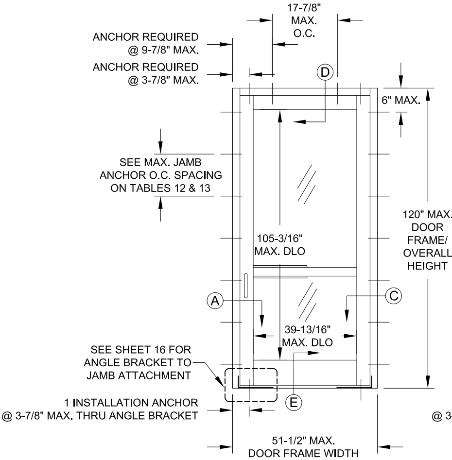
TYP. ELEVATION OF SINGLE DOOR WITHOUT TRANSOM
