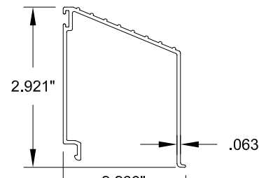
18 3" THRESHOLD COVER (3" TOTAL SILL HEIGHT)
