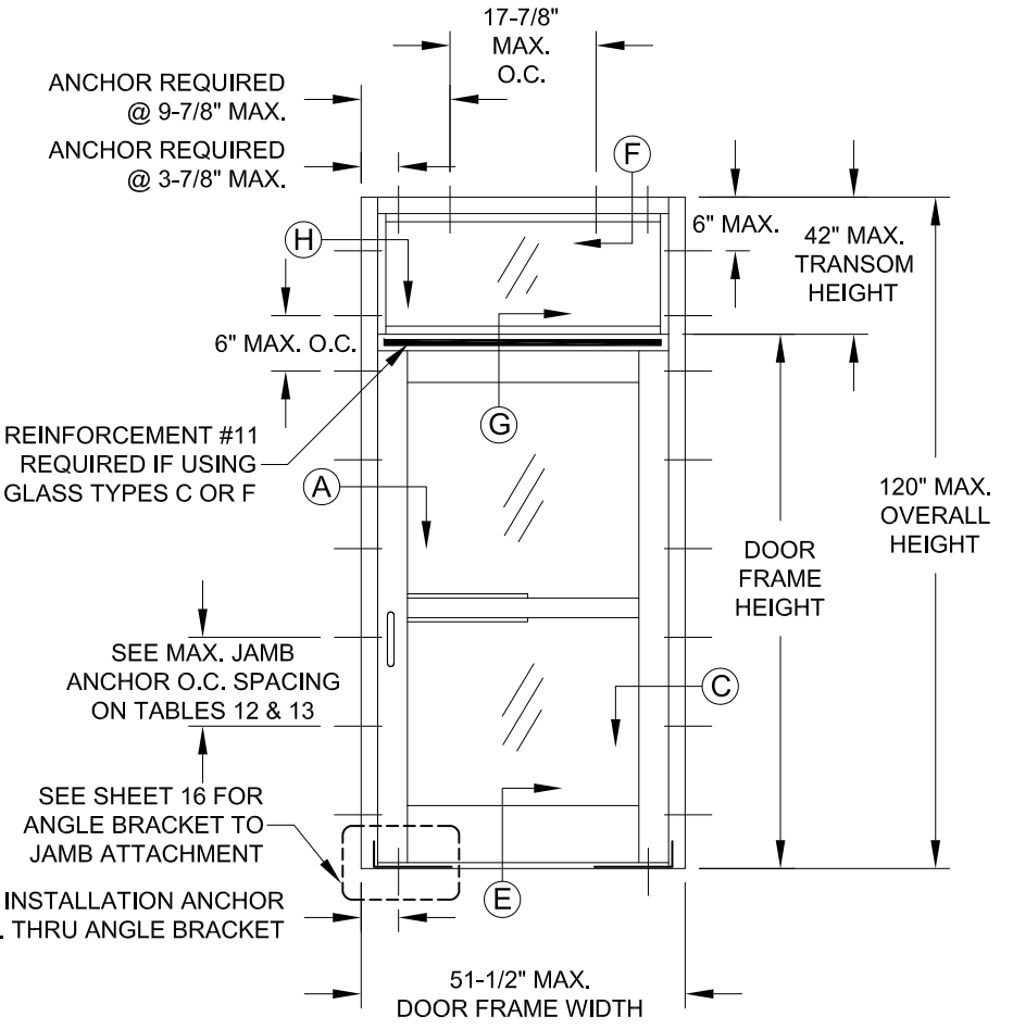
TYP. ELEVATION OF SINGLE DOOR WITH TRANSOM
